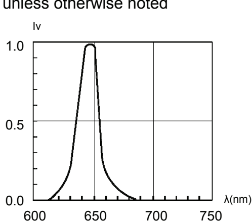
Fig. 1 Relative Luminous Intensity vs. Wavelength @ 20mA
