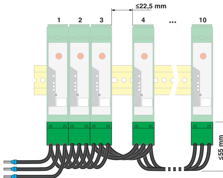
Application drawing
