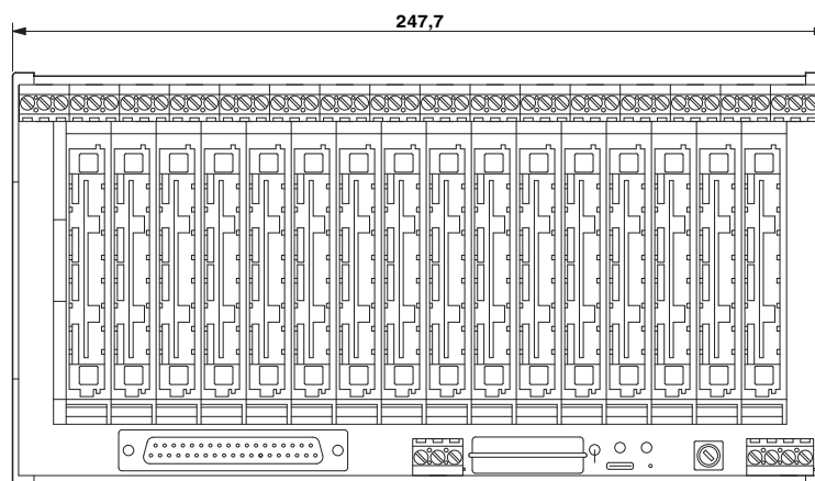
Dimensional drawing
