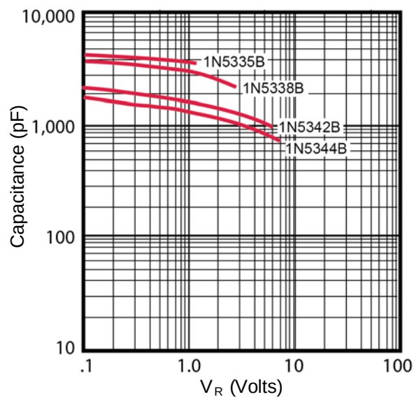
FIGURE 2 Typical Capacitance vs. Reverse Voltage for 5 Watt Zeners
