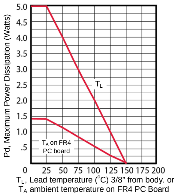
FIGURE 1 Power Derating Curve
