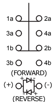
DPDT ON (OFF) / OFF (ON) CONTACT CONFIGURATION
