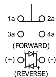
SPDT ON (OFF) / OFF (ON) CONTACT CONFIGURATION
