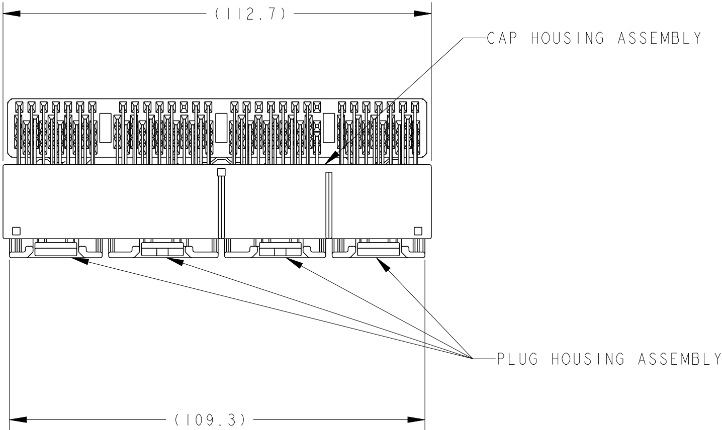
CAP HOUSING ASSEMBLY & PLUG HOUSING ASSEMBLY ENGAGEMENT VIEW CAP HOUSING ASSEMBLY & PLUG HOUSING ASSEMBLY 嵌合図
