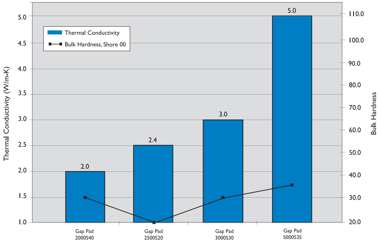
Gap Pad "S-Class" Thermal Conductivity vs. Hardness
