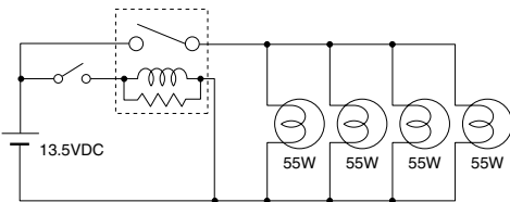
Circuit
