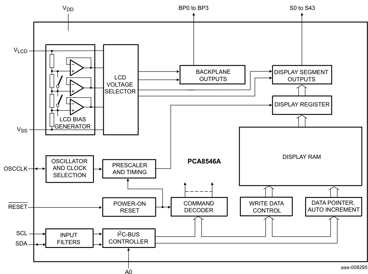
Fig 1. Block diagram of PCA8546A
