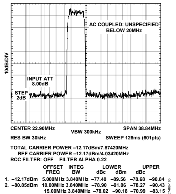
Figure 65. AD9117 ACLR One-Carrier, 3.3 V
