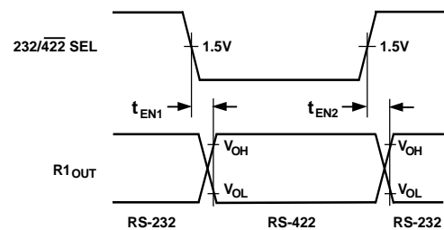
Figure 6. RS-232/RS-422 Receiver Enable Timing
