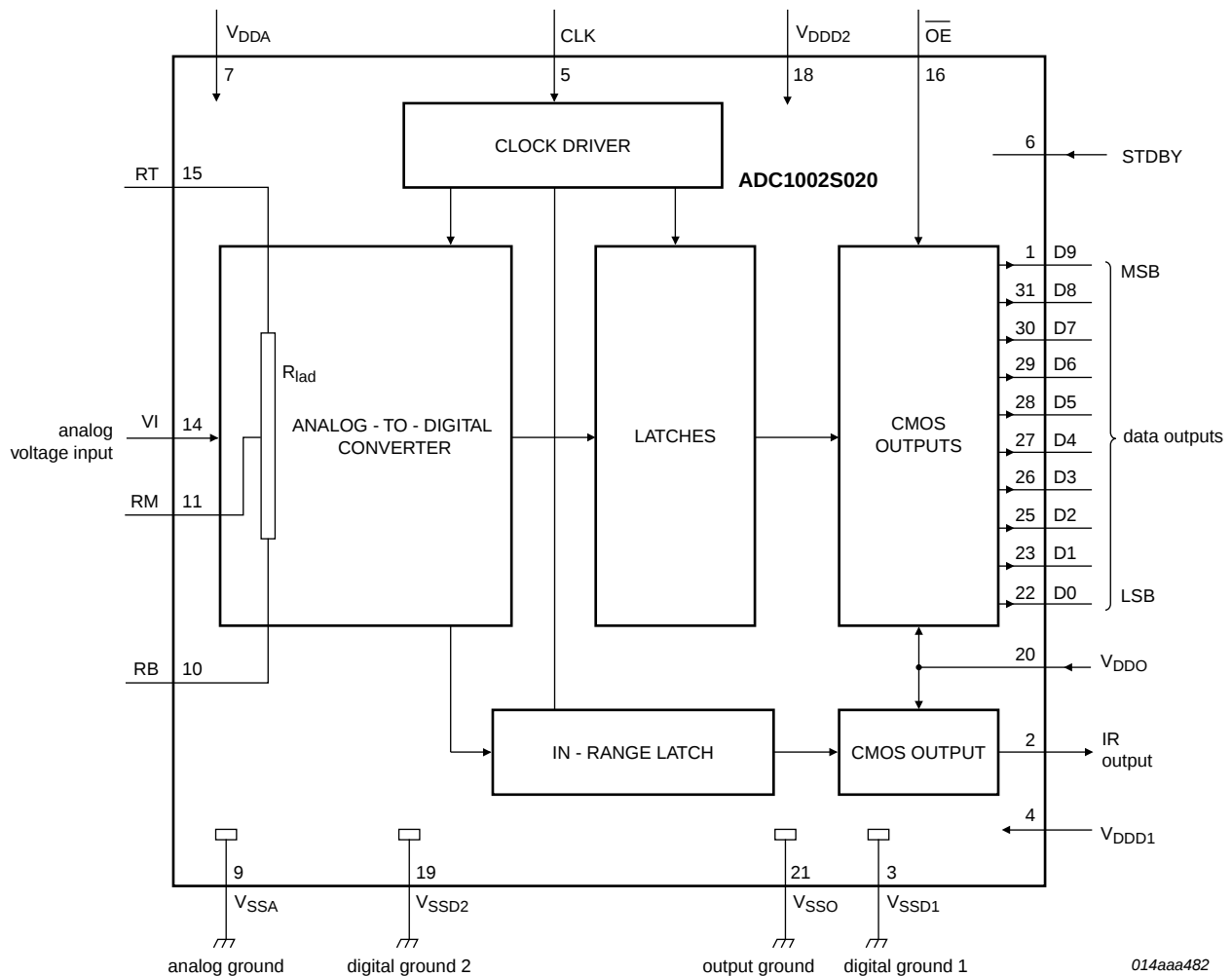
Fig 1. Block diagram
