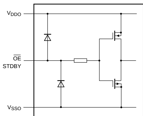
Fig 12. \overline{\text{OE}} and STDBY inputs
