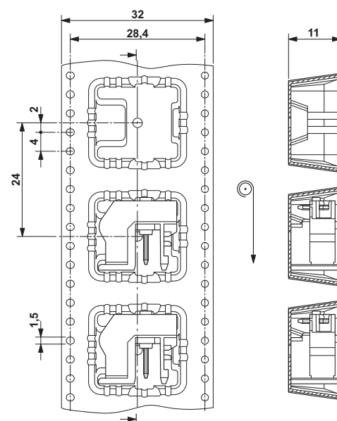
Dimensional drawing
