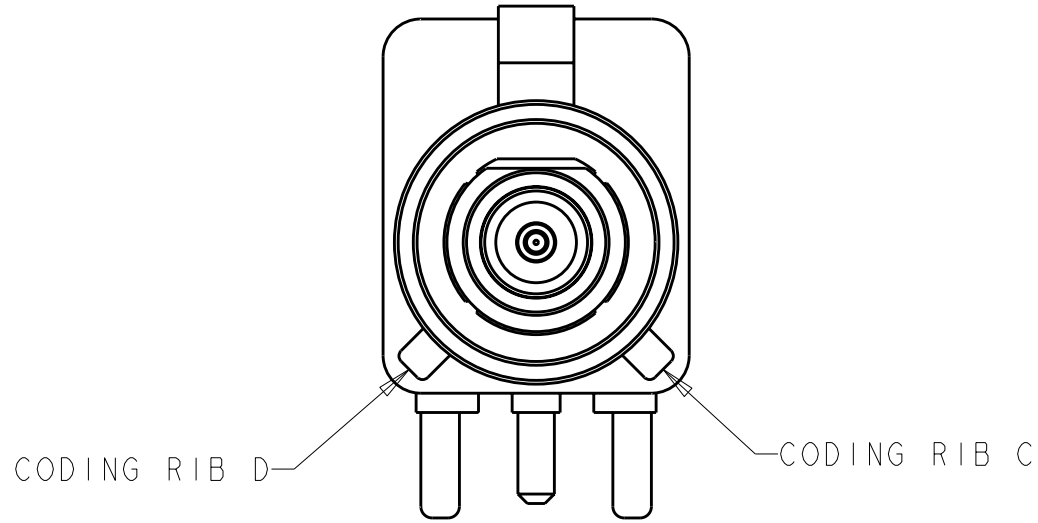
DETAIL K
