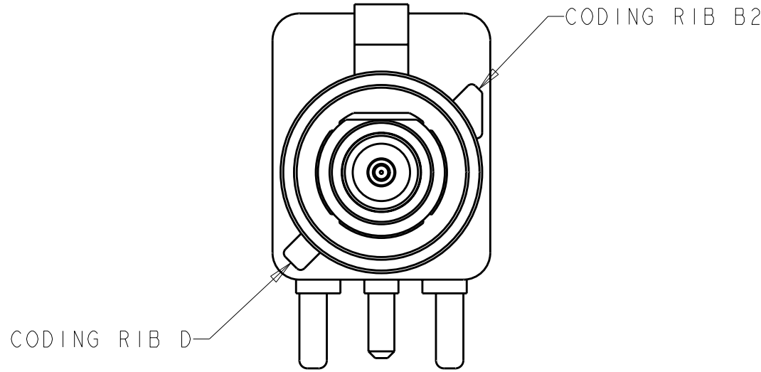
DETAIL I
