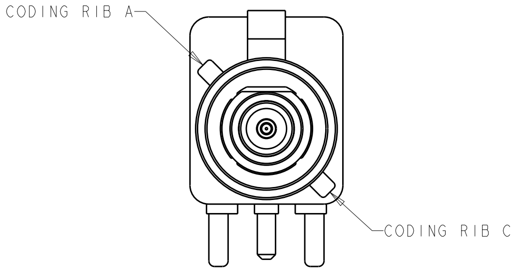
DETAIL C
