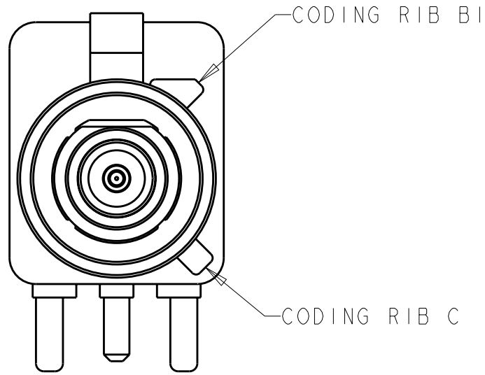
DETAIL F
