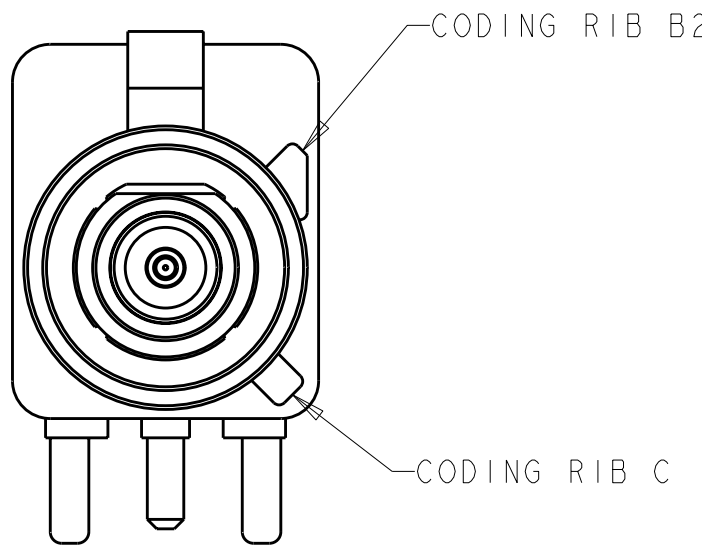
DETAIL H
