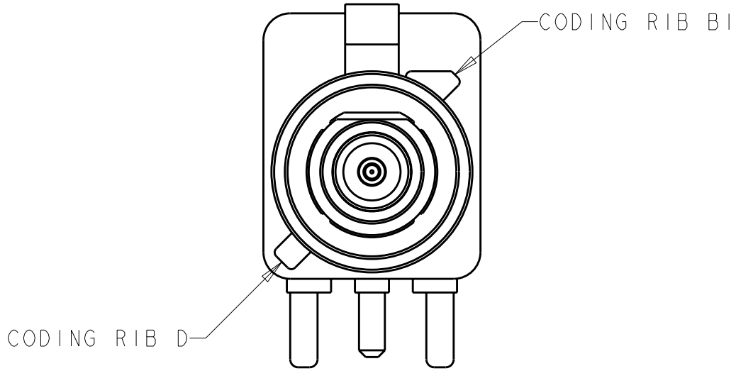
DETAIL G
