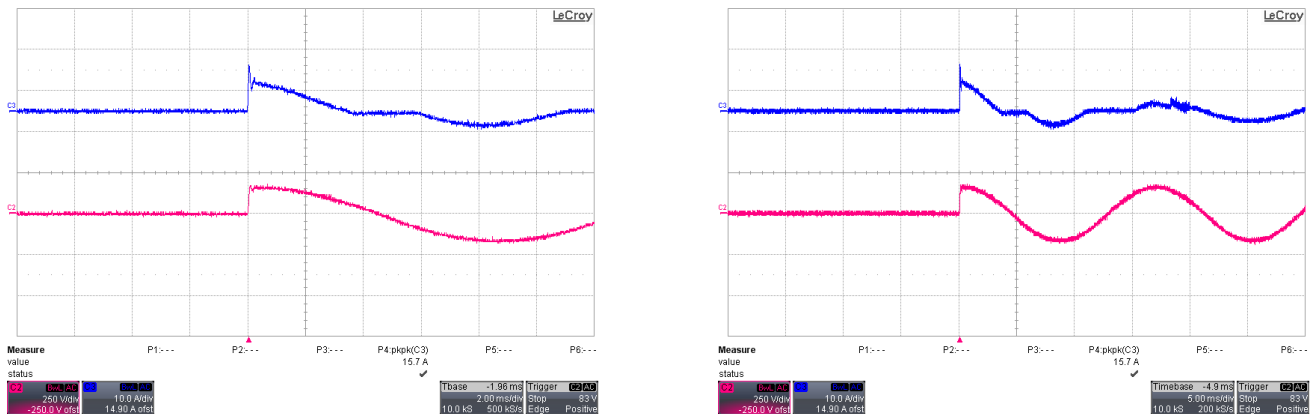
Figure 2: Inrush current, V_{in} = 115\text{Vac} , 90^\circ CH2: V_{in} (250V/div), CH3: I_{in} (10A/div)
