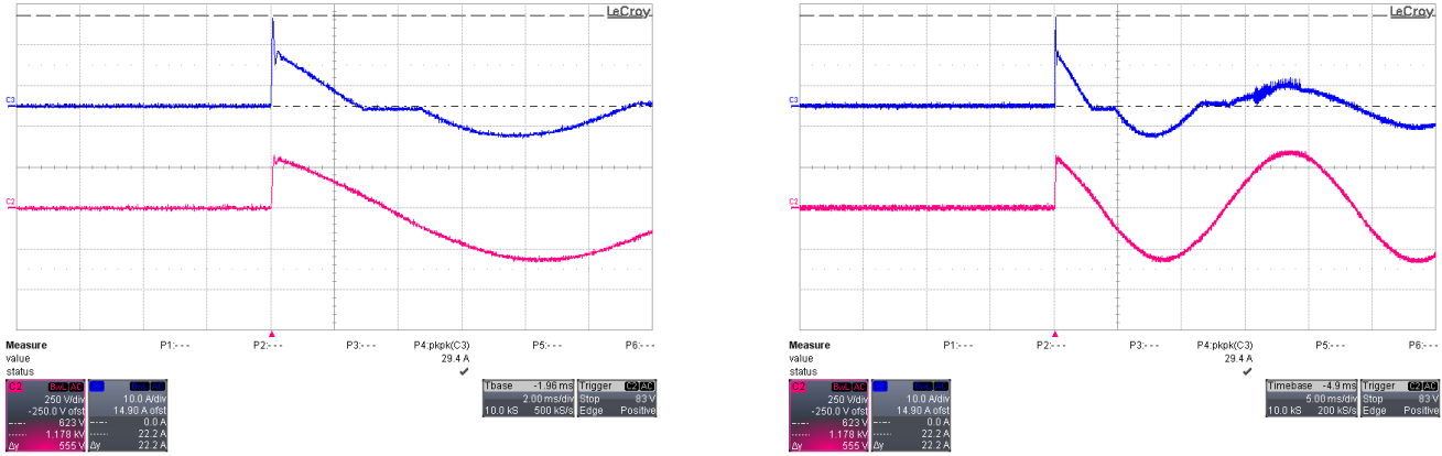
Figure 3: Inrush current, V_{in} = 230Vac , 90^\circ CH2: V_{in} (250V/div), CH3: I_{in} (10A/div)
