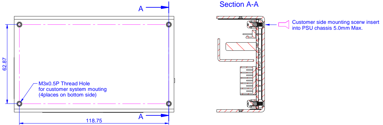
Figure 20: Bottom view 2
