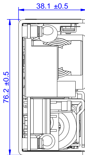
Figure 21: Front view
