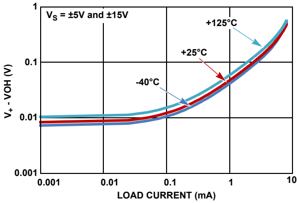
FIGURE 23. OUTPUT OVERHEAD VOLTAGE HIGH vs LOAD CURRENT, -40°C to +125°C, V_S = \pm 5V AND \pm 15V
