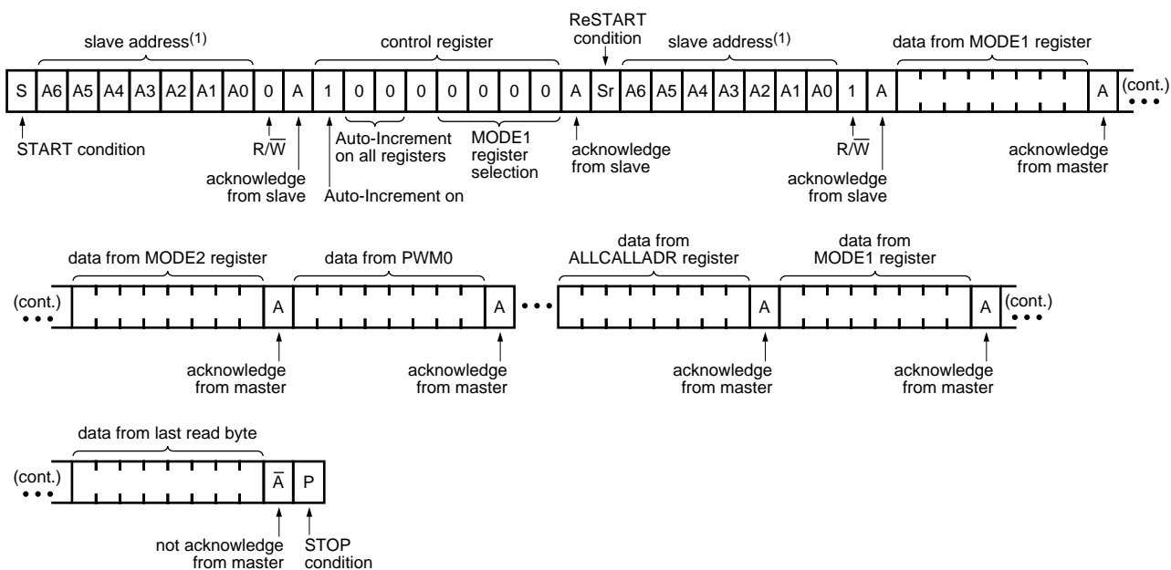
Fig 19. Read all registers using the Auto-Increment feature
