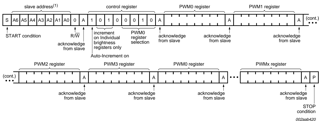
Fig 18. Multiple writes to Individual Brightness registers only using the Auto-Increment feature
