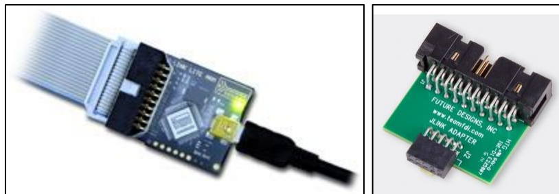
Figure 3: J-Link Hardware
