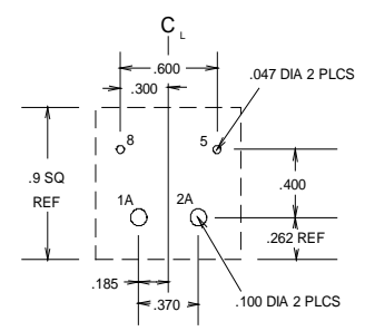
MOUNTING HOLE PATTERN TOP OF PCB
