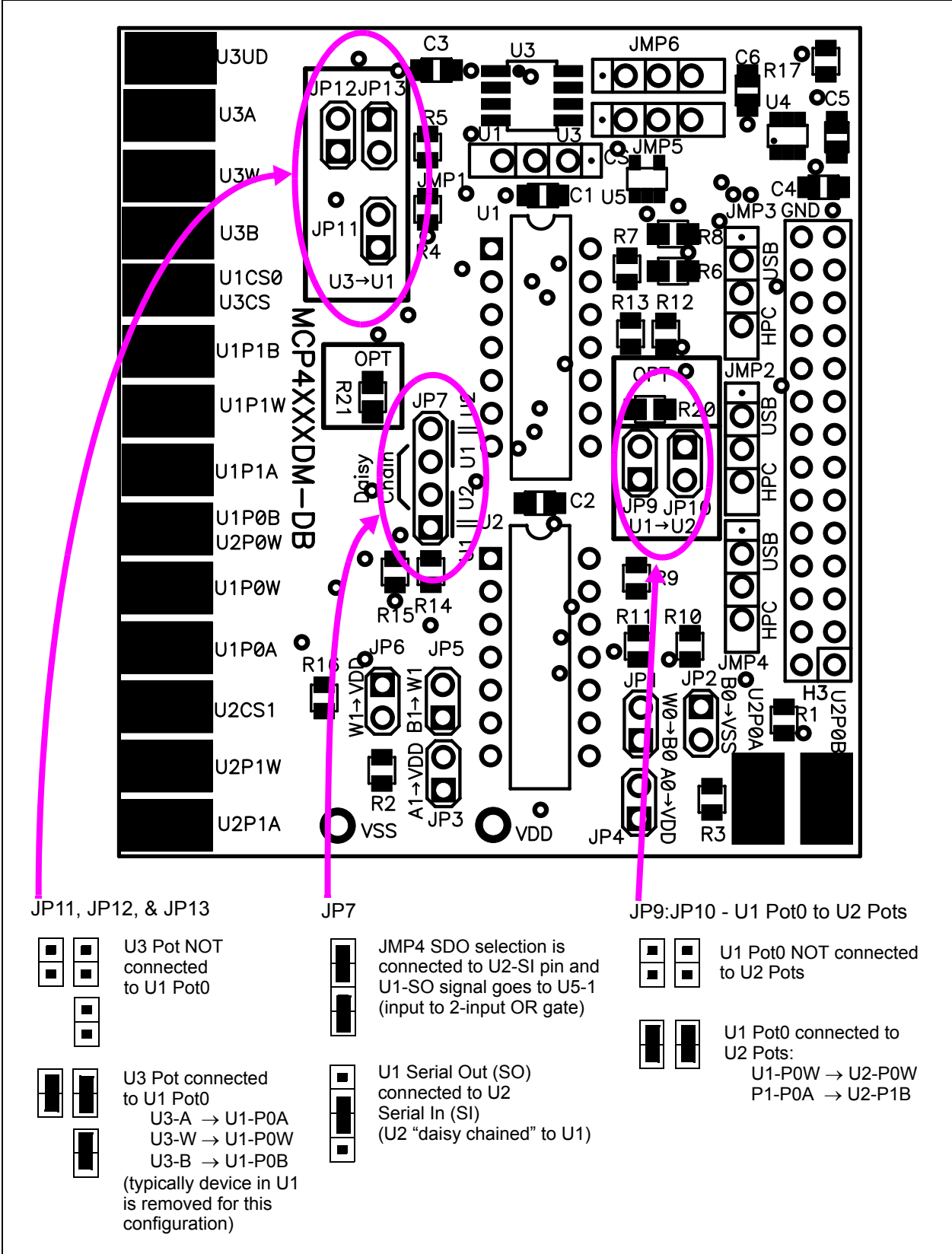
FIGURE 2-5: Jumper JP7, JP9, JP10, JP11, JP12, and JP13 Configurations.
