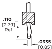
Straight and Right-Angle Post with Retentive Legs
