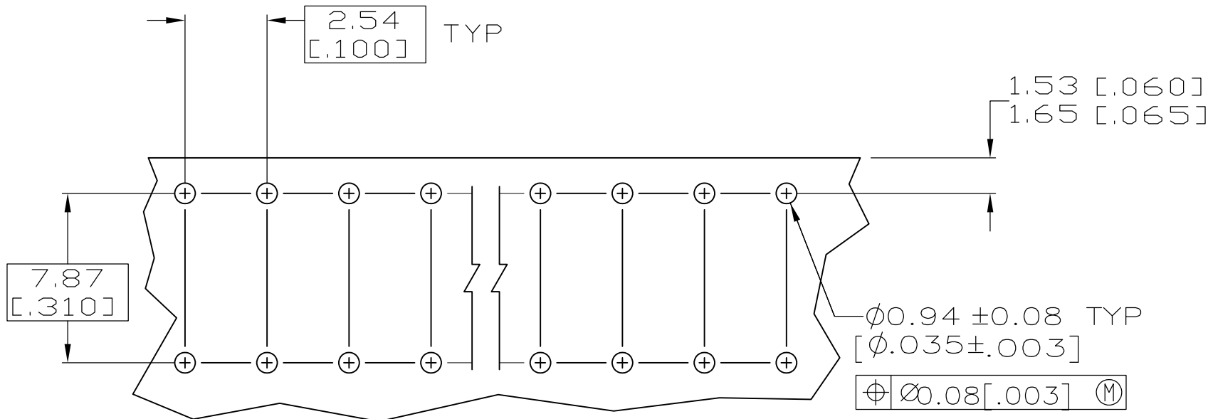
RECOMMENDED HOLE LAYOUT SCALE 4:1
