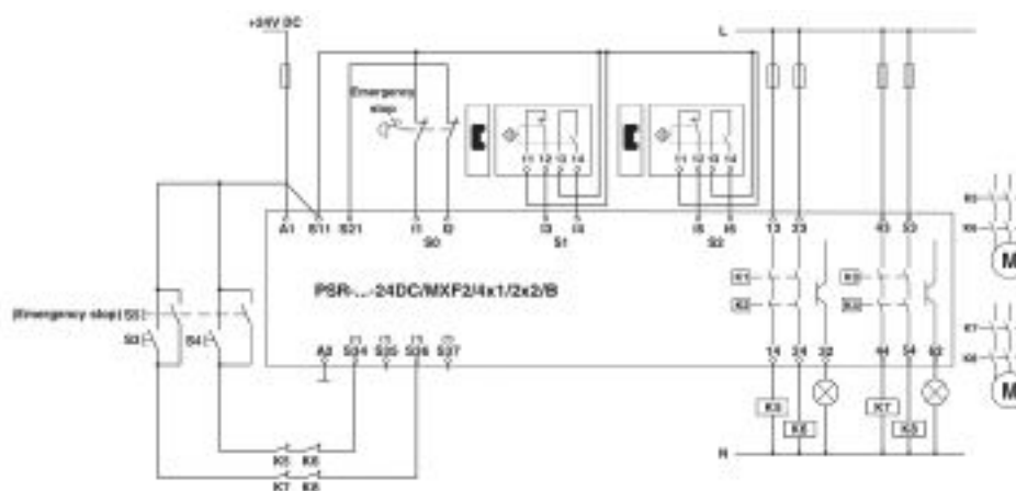
Circuit diagram
