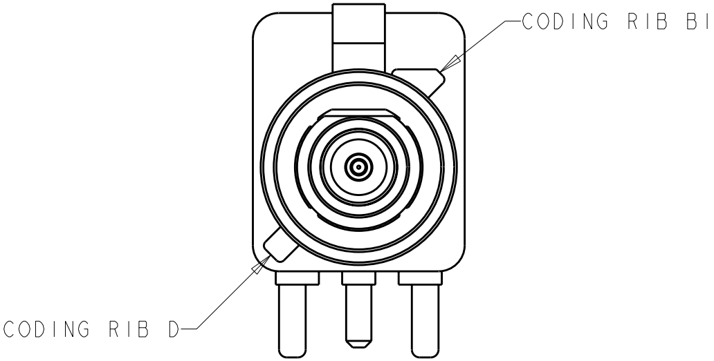
DETAIL G
