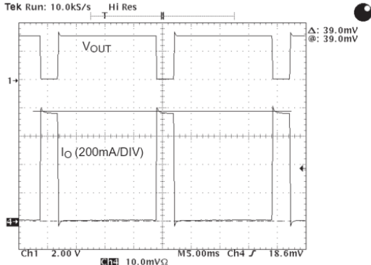
Fig. 4: Current Limit
