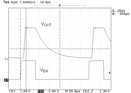
Fig. 5: Turn-On Time, R_{LOAD}=50\Omega (60mA)
