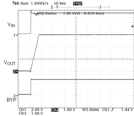
Fig. 17: Fast V_{IN} = 1000 \mu F Output Load
