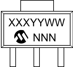
3-Lead SOT-89
