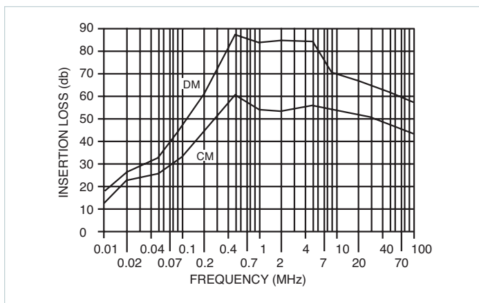
Figure 13.13 — HAM filter insertion loss vs. frequency
