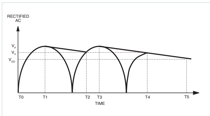
Figure 12.3 — AC waveforms
