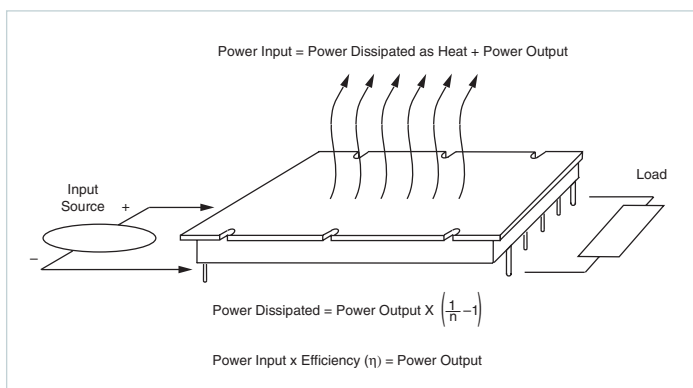
Figure 20.1b — Dissipated power
