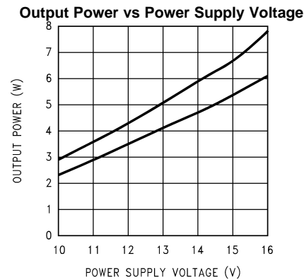
R_L = 4\Omega , SE operation, f_{IN} = 1kHz , both channels driven and loaded (average shown), at (from top to bottom at 12V): THD+N = 10%, THD+N = 1%
