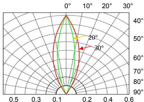
Fig. 2 Directivity Radiation Diagram
