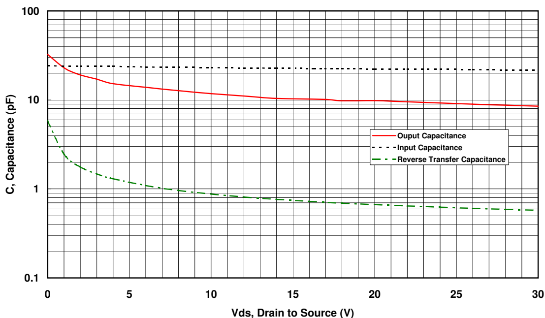
Figure 6 – Typical CV Characteristics.
