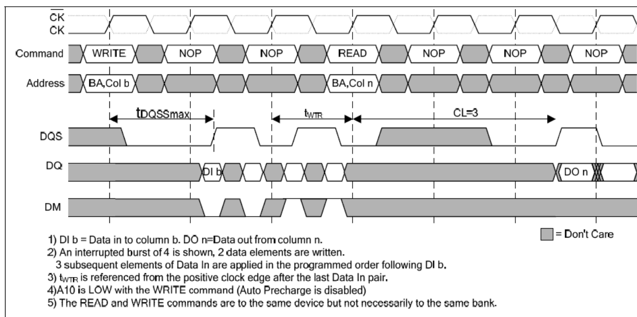
Figure 29 — Interrupting Write to Read
