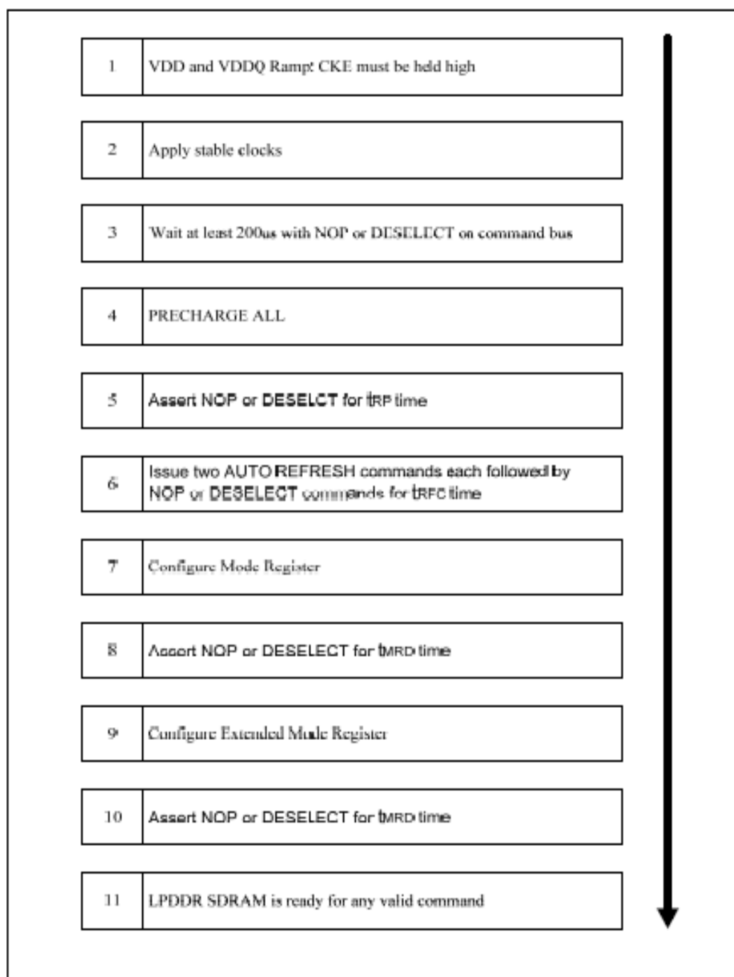
Figure.4 — Flow Diagram
