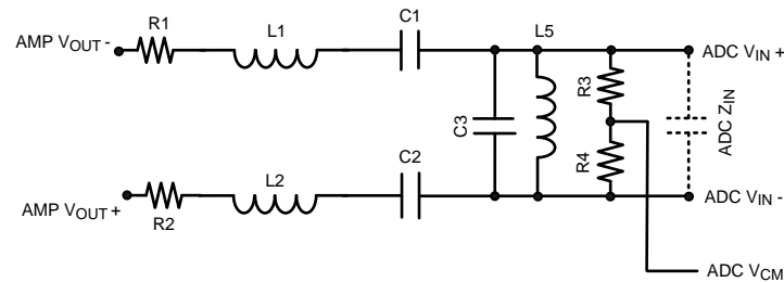
Figure 44. ADC Noise Filter Schematic
