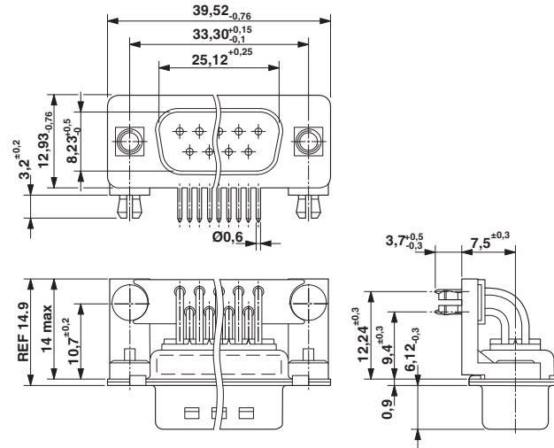
Dimensional drawing
