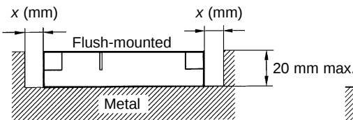
Flush-mounted in metal casing Surface-mounted on metal
