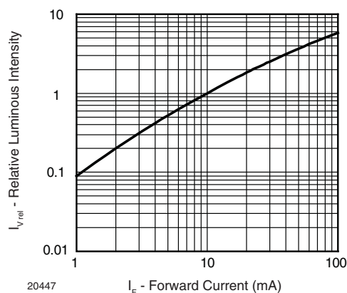
Fig. 5 - Specific Luminous Flux vs. Forward Current
