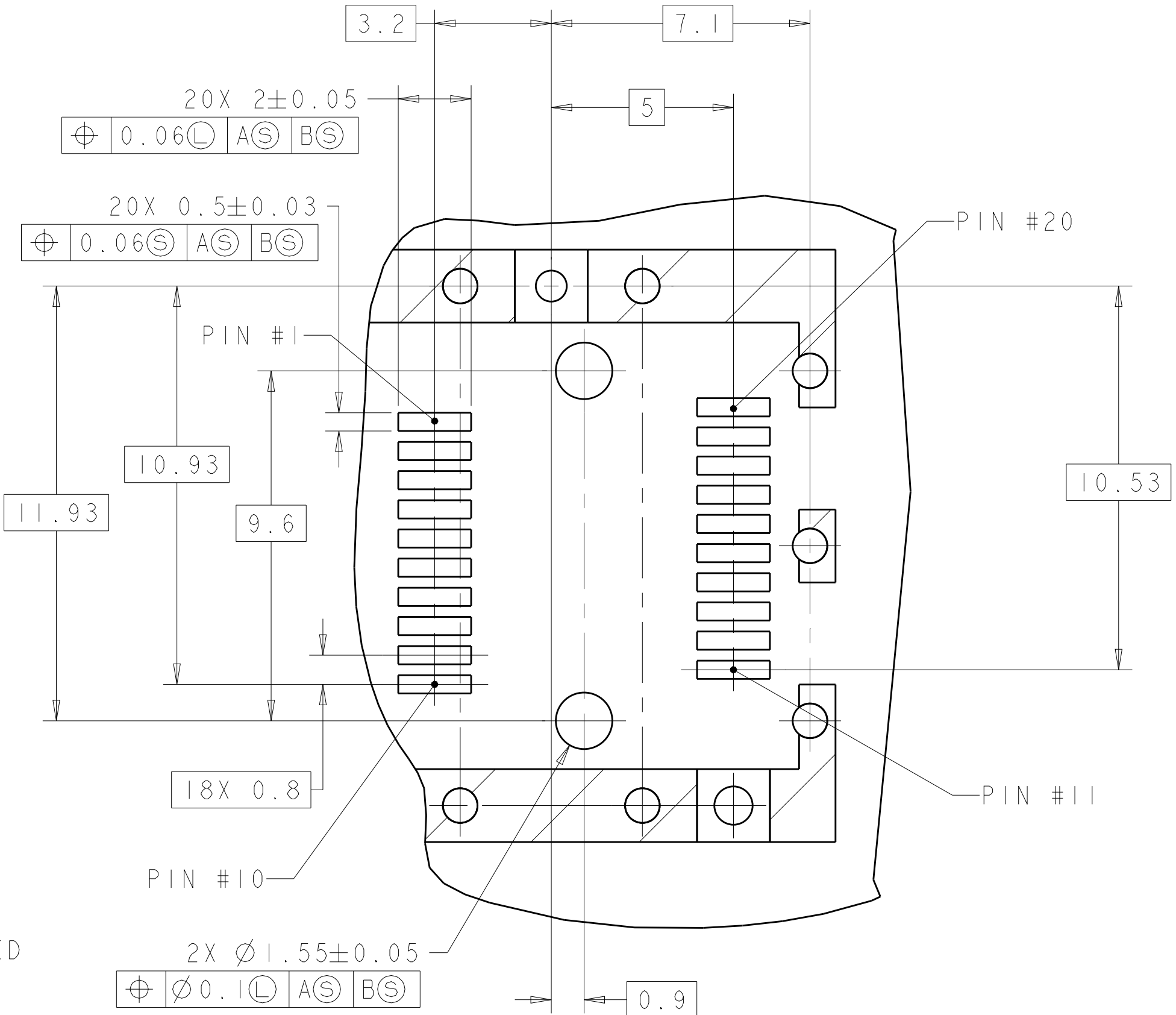
DETAIL D SCALE 8:1
