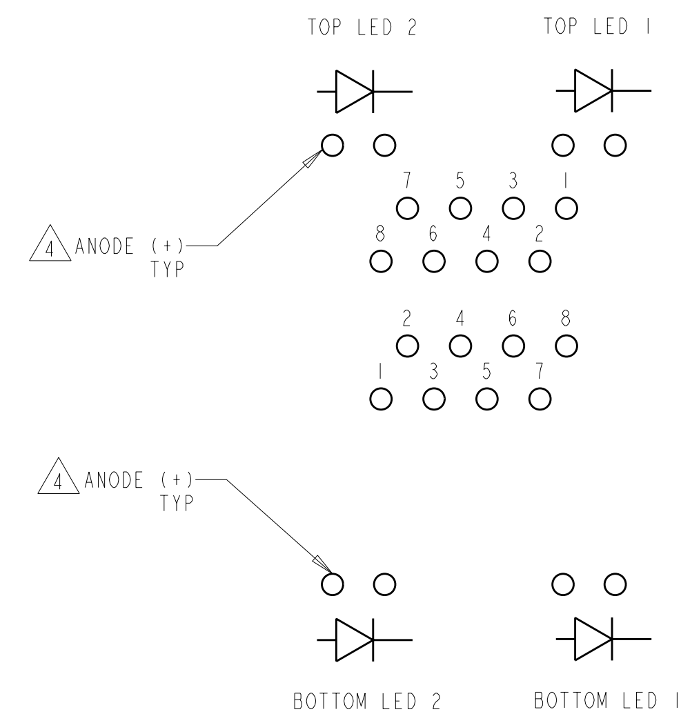
SCHEMATIC FOR 6116314-1, -2, -3 & -13 SCALE 4:1
