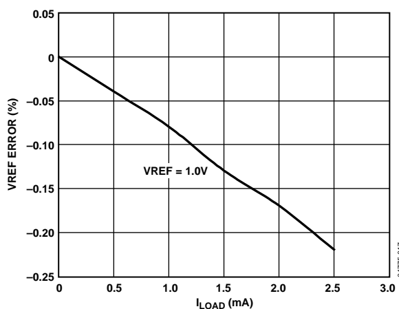
Figure 50. VREF Accuracy vs. Load
