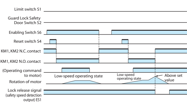
Timing Chart for Maintenance Mode (M1: OFF, M2: ON)
