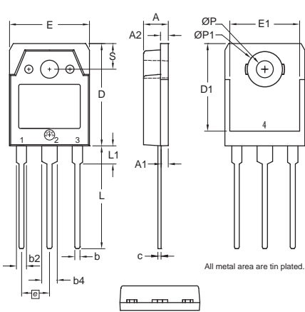
X017a TO-3P Weight = 5.5 g
