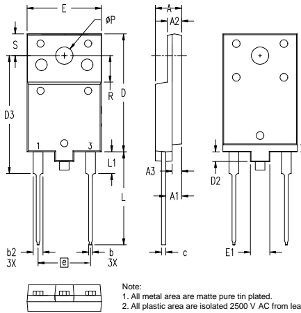
X017d TO-3PFP Weight = 5.4 g
