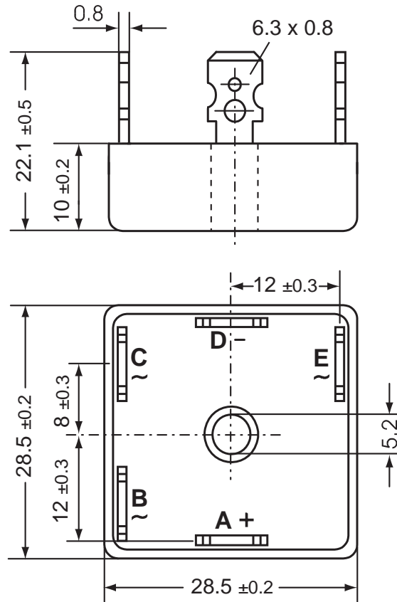
X117b FO-F-B Weight = 45 g
