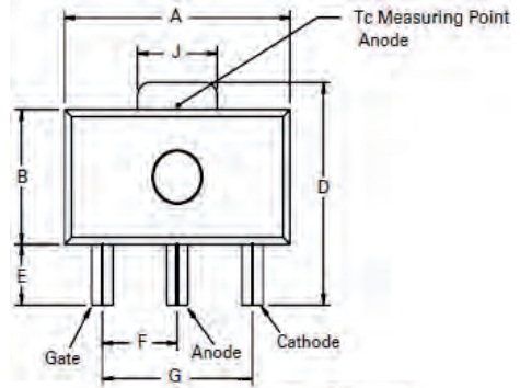
L016 SOT-89 Weight = 0.045 g
