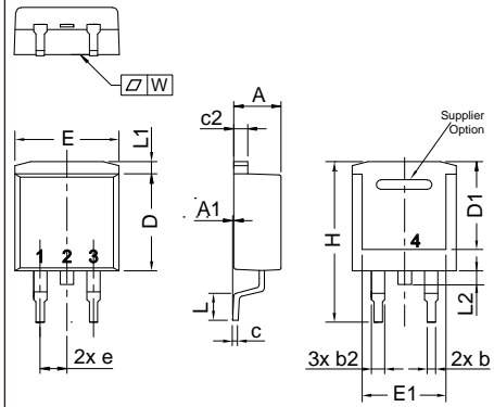
X011b TO-263 AB (D 2 PAK) Weight = 1.5 g
