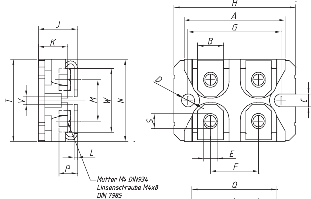
L027a SOT-227 B miniBLOC Weight = 29 g
