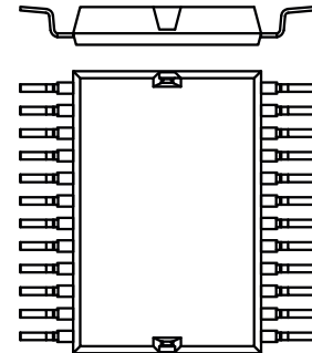
MTI...WX...GD; MTC...X...TGD; GMM... SURFACE MOUNT DEVICE
