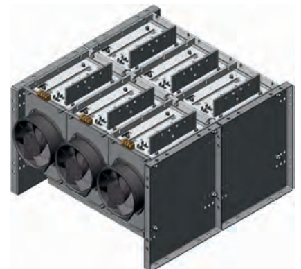
Figure 6 Weight 60 kg
