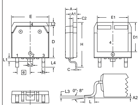
X019 TO-268 AA (D 3 PAK) Weight = 4 g
