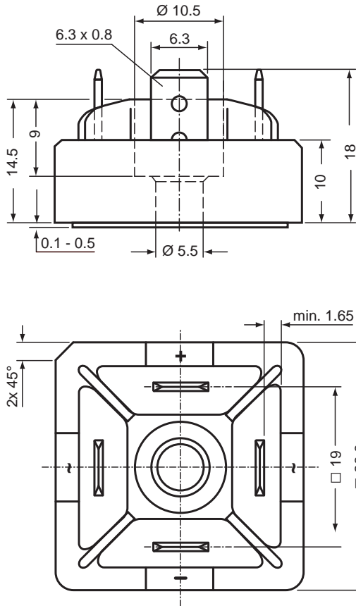
X117a FO-F-A Weight = 45 g
