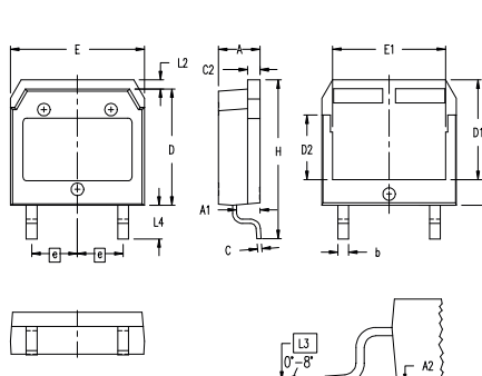
X019a TO-268 AA (D 3 PAK HV) Weight = 4 g
