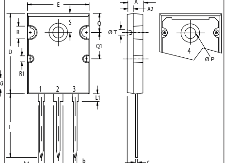
X020a TO-264 AA Weight = 10 g
