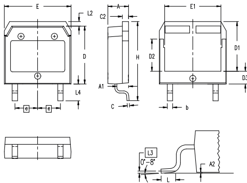
L019a TO-268 AA (D 3 PAK HV) Weight = 4 g
