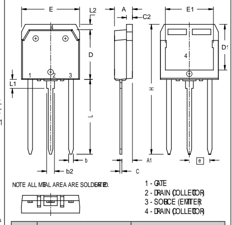
X018 TO-268 I 3 PAK Weight = 4.5 g
