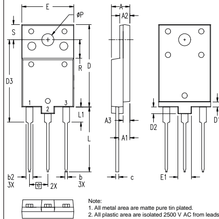
X017c TO-3PFP Weight = 5.5 g
