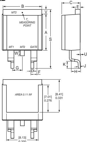
L011b TO-263AB Weight = 1.5 g
