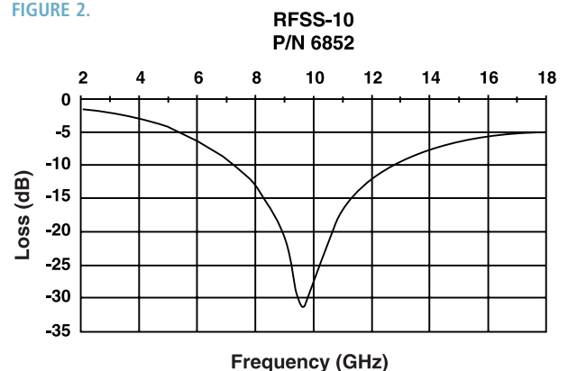
▲ Salisbury Screen resonant absorber at 10GHz.
