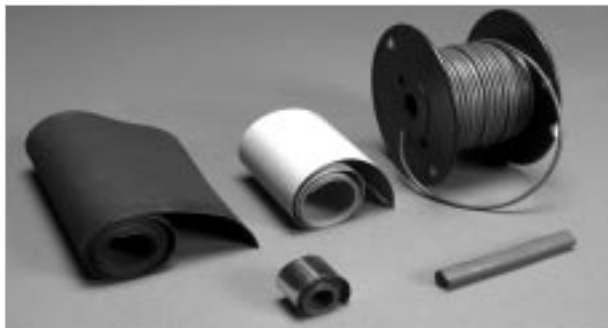
▲ Thermoplastic products include microwave absorbing tapes, string and hot-melt glue sticks.
