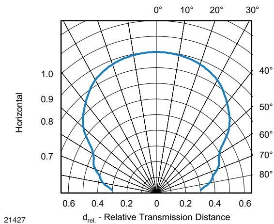
Fig. 3 - Horizontal Directivity
