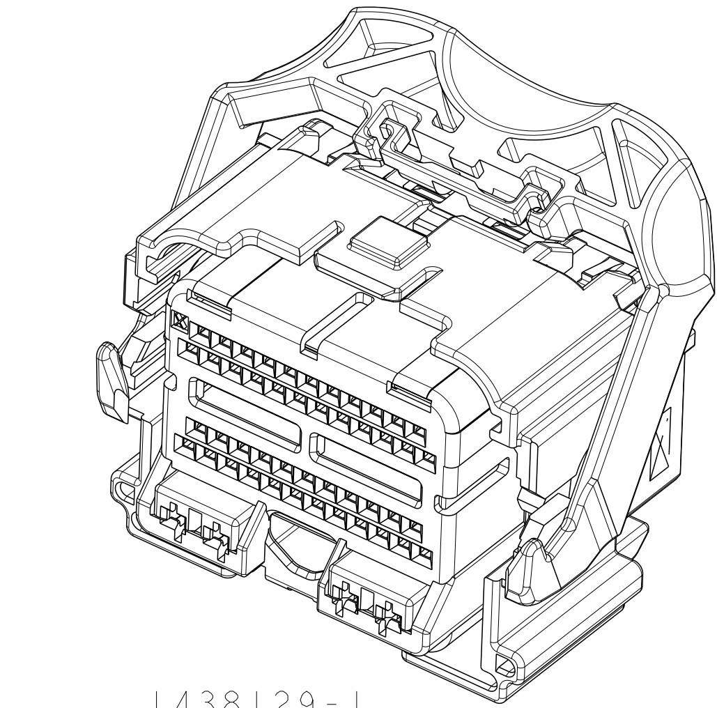
1438129-1 SHOWN WITH SPACER IN SEATED POSITION
