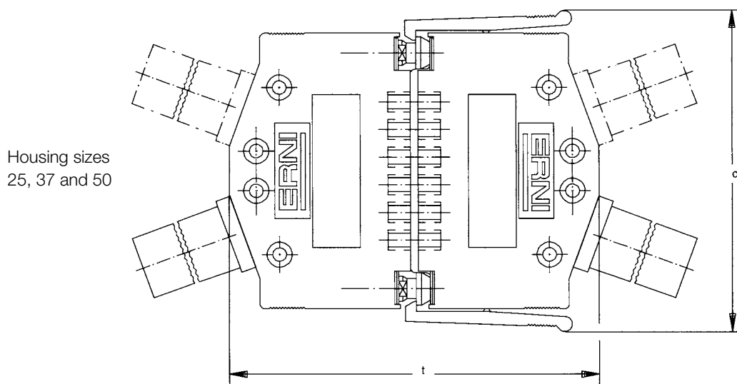
Dimensions of cable coupler cable connector housing Series KSG 185
