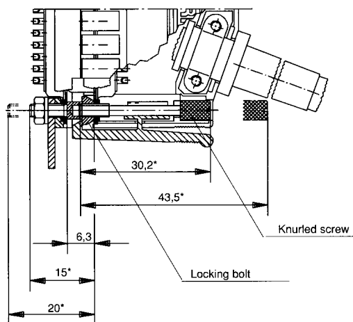
Dimensions of cable coupler cable connector housing Series KSG 185
