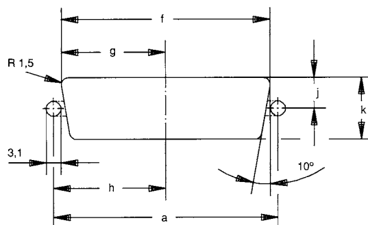
Dimensions of panel cutout
