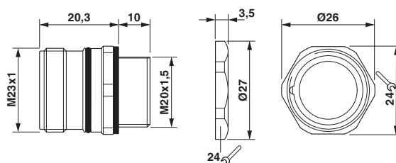
Dimensional drawing
