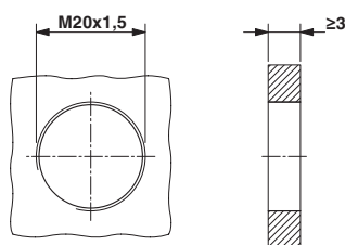
Dimensional drawing
