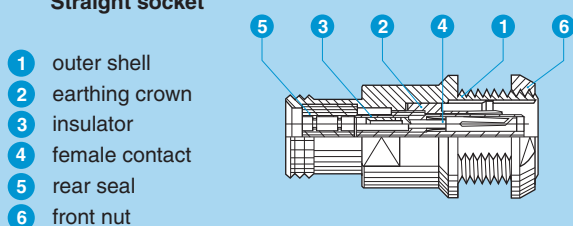
Straight socket
