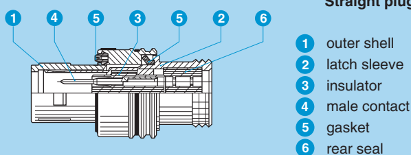
Straight plug
