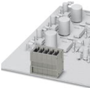
ST-COMBI receptacle, plug-in direction vertical to the PCB, pitch: 5.2 mm, no. of positions: 7
