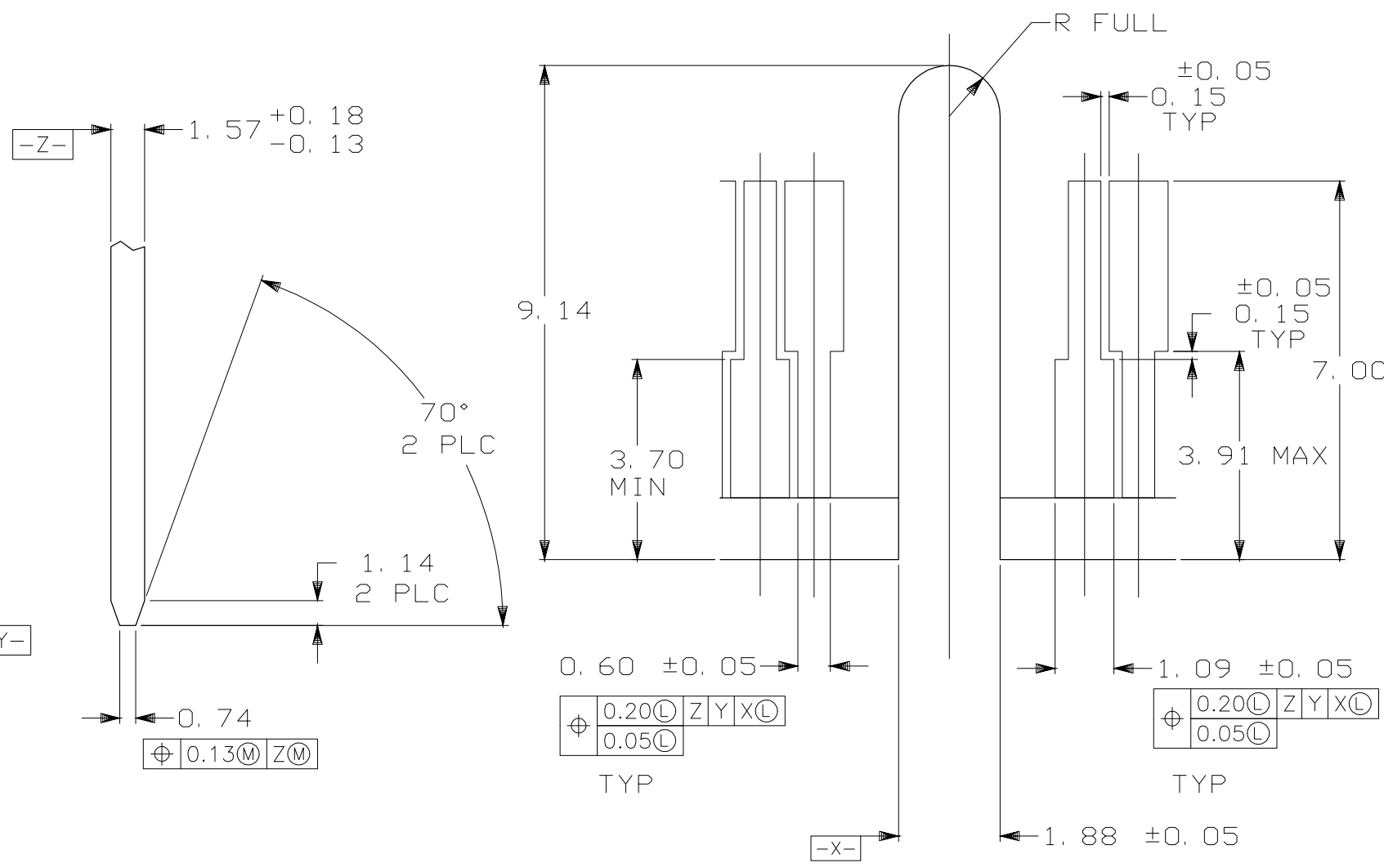
DETAIL D SCALE 10:1
