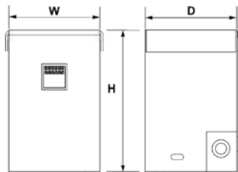
Style 2 - Non-Encapsulated
