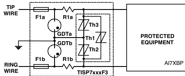
Figure 20. Protection Module
