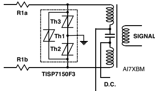
Figure 21. ISDN Protection
